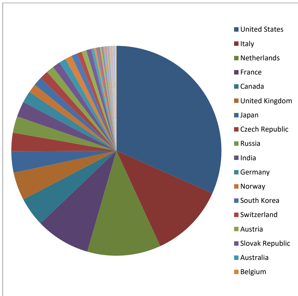
Graph 2: GL Countries
