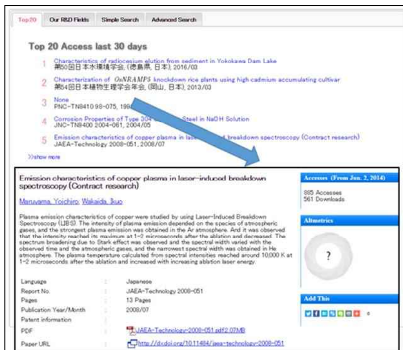
Figure 10 “Top 20” tab
