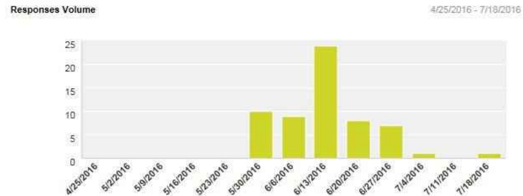
Figure 1: Response Volume
